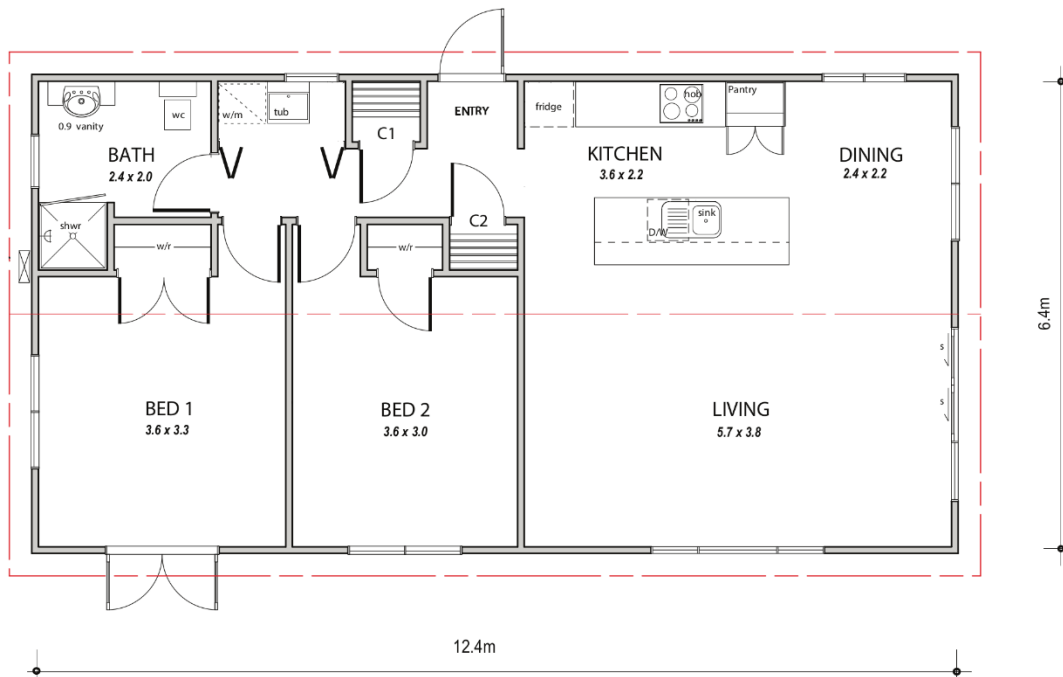
Figure 1 - Sample plan of finished layout
